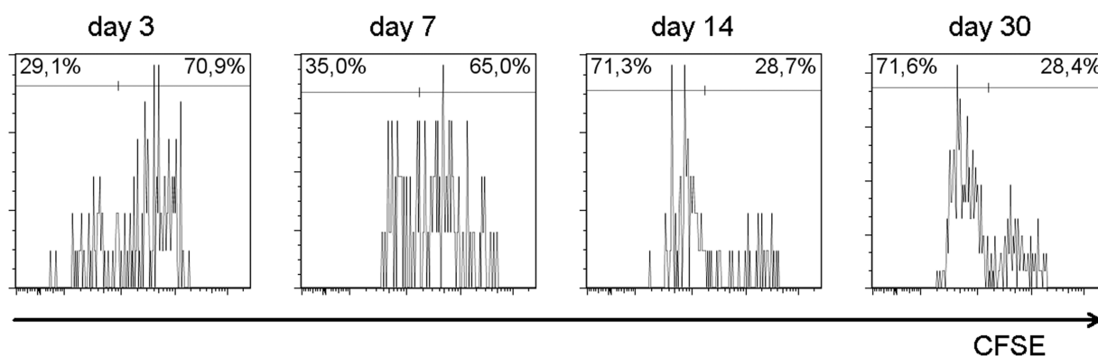
Figure 1 Behaviour of adoptively transferred antibody-secreting cells (ASCs) in the bone marrow (BM) of recipient Rag1 -/- mice. For this analysis, ASCs isolated from the spleens of NZB/W mice were labelled with carboxyfluoresceinsuccinimidyl ester (CFSE) prior to transfer. CFSE is a membrane-permeable, fluorescein-based dye that crosslinks to intracellular proteins. We used it to track the cell division of transferred ASCs in BM in vivo as each cell division results in the progressive halving of the fluorescence intensity of the dye in cells. Histogram plots of BM ASCs gated for CD138 + and intracellular kappa + cells in recipient Rag1 -/- mice showed a loss of CFSE intensity from days 3 to 14 after transfer but no further change in CFSE intensity after that. The persistence of CFSE labelling is indicative of the absence of proliferation.
